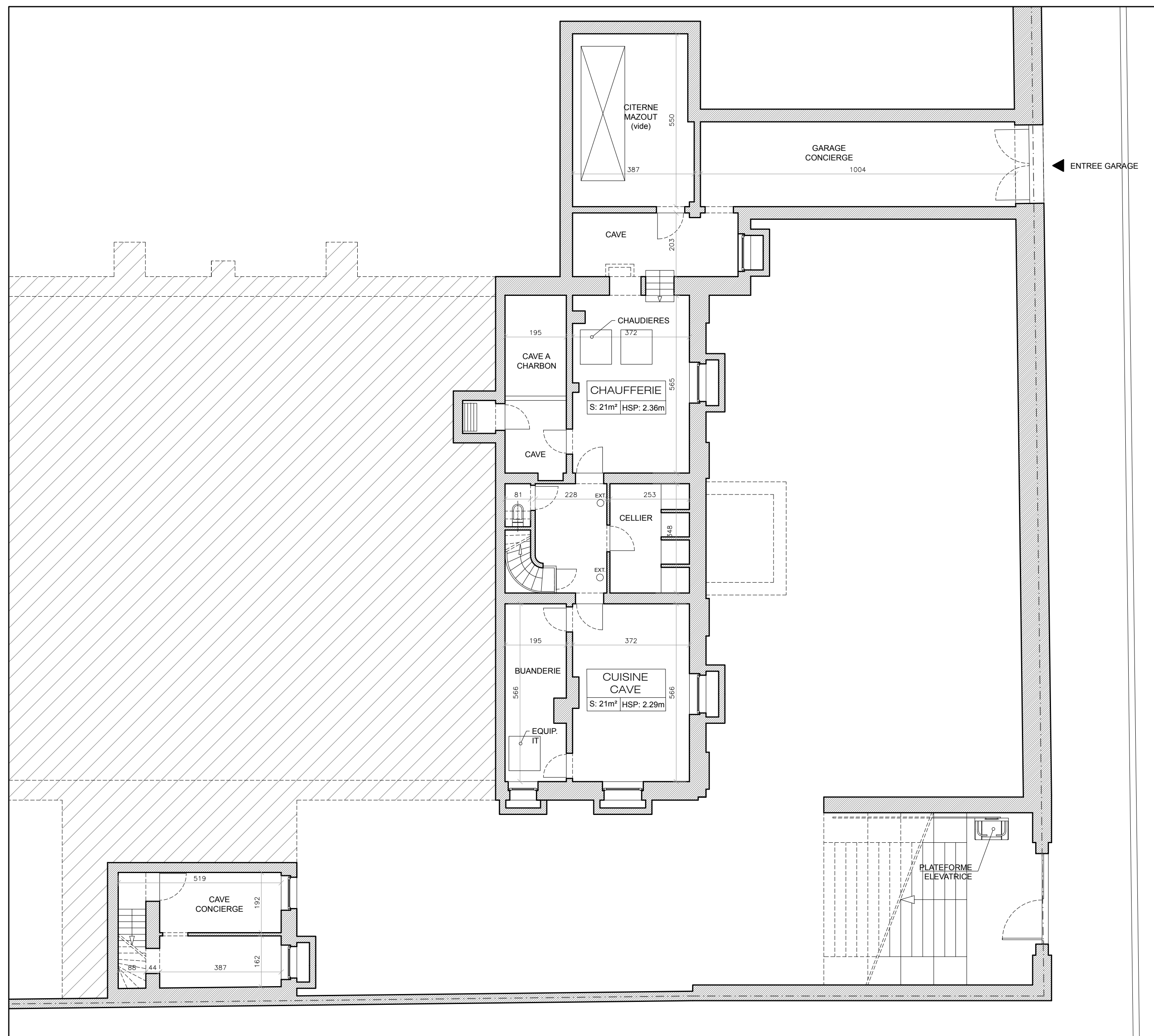
PLAN CAVES (1/100)
